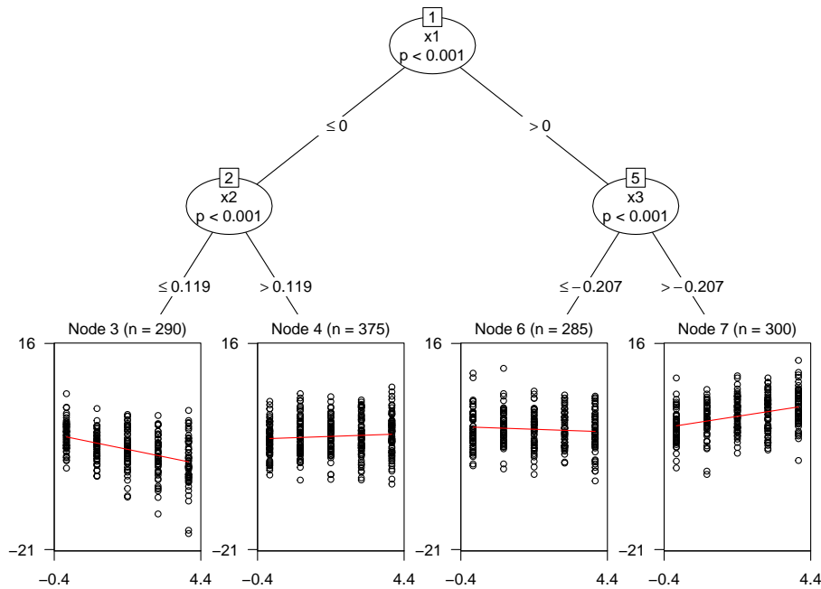
Figure 8: Linear mixed-effects model tree with growth curve models in the terminal nodes.
