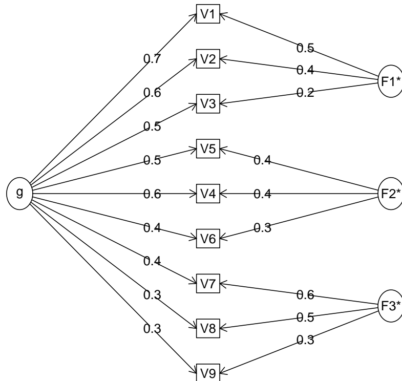
Figure 13: A bifactor solution for 9 simulated variables with a hierarchical structure. In the case of these simulated 9 variables, the amount of variance attributable to a general
